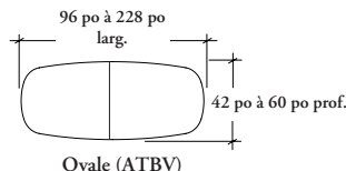
Ovale (ATBV)
