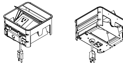
Wire Pass through on two sides 1 1/8" high
