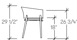
Africa Chair, Armchair (VMAFB)
