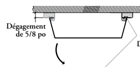
Configuration double
