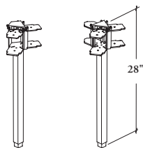
Two-Way – Double-Sided Beam (V)
