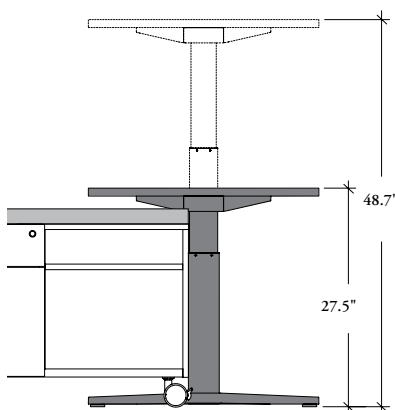
Navigate Cityline Restricted Electric Base Mechanism (9M)
