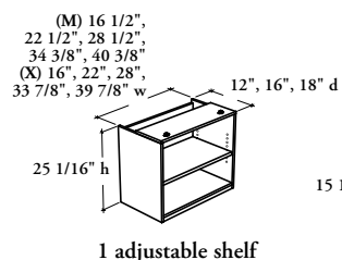
Bookcase – Secondary Desk – End Position (BSSOM, X)
