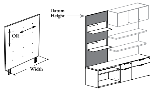
Mounting Style (K)
