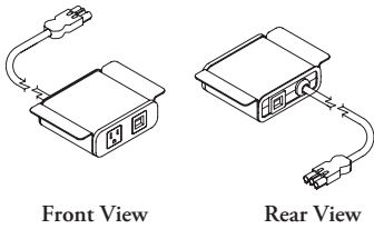
Front View Rear View 1 Power / 1 USB A+C (65W) / 1 Rear Power (shown))
