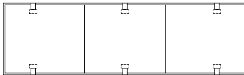
Edge USB or Undersurface Modules for 204" - 240" (6 modules)
