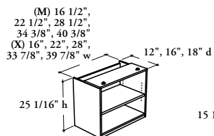
Bookcase – Secondary Desk – End Position (BSSOM, X)
