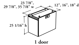
Recycling/Waste Cabinet – Secondary Desk – Center Position (BSSRWC)
