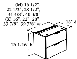
Lateral File – Secondary Desk – End Position (BSSLM, X)
