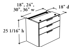
Stretch Pedestal – Secondary Desk – Center Position (BSSPC)
